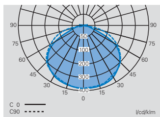
Polar curve Planete 400
