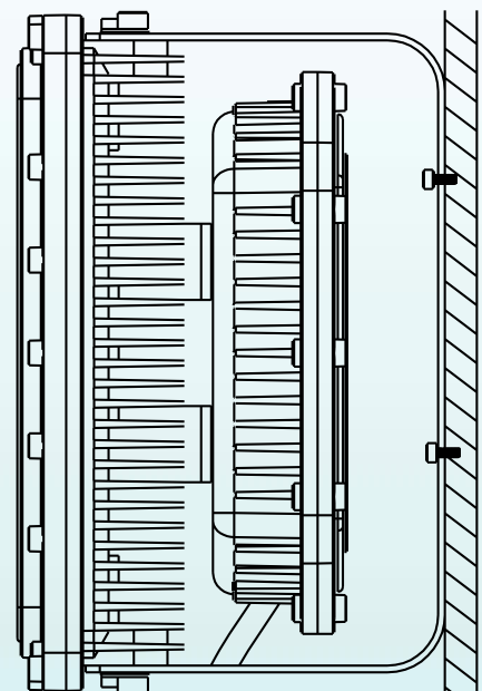
Wall Bracket Mounting
