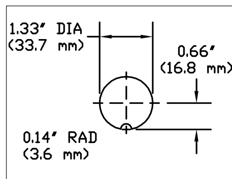
Figure 4. Switch mounting hole.
