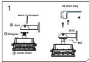
1. Tighten part 2 and assembly 1, and fix the M3 screw/install arm to the adaptor, tighten the M10 via 16F allen key.
